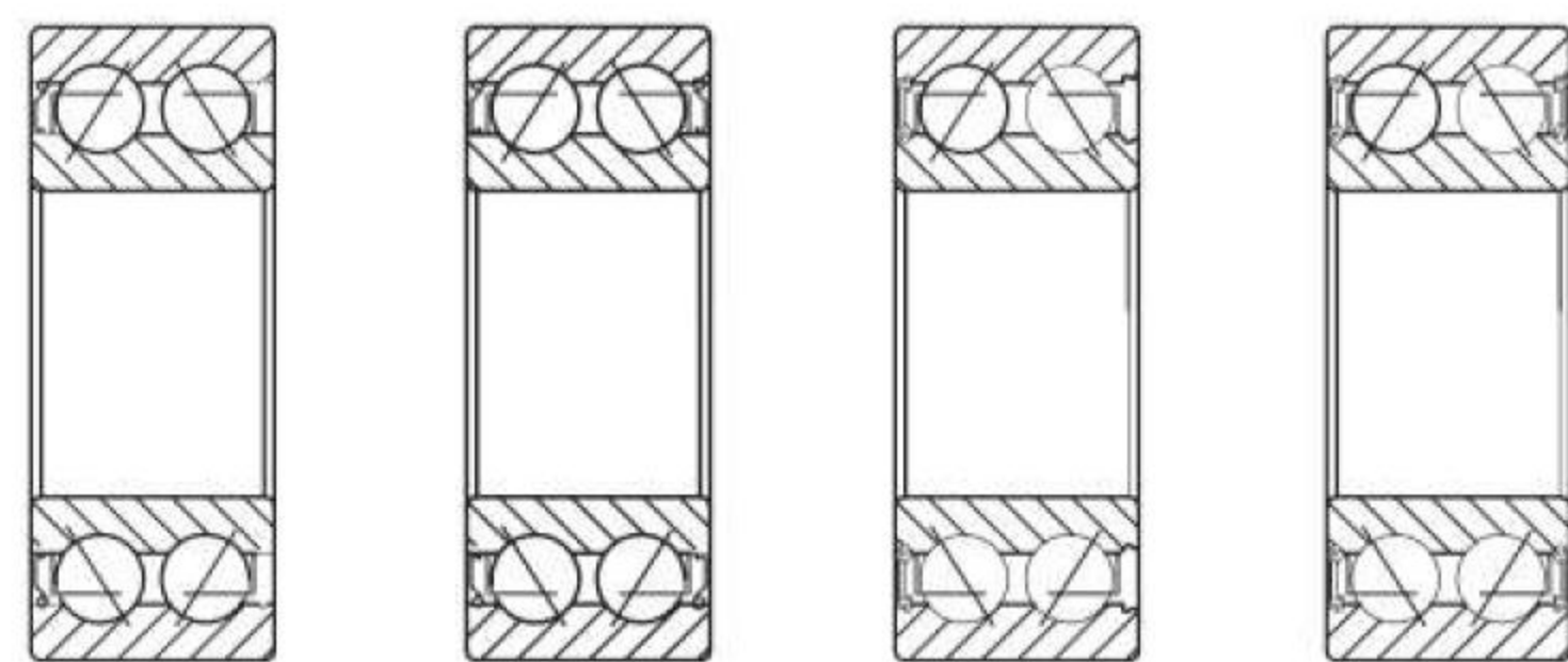
Shield on one side -Z Shield on both sides -2Z Seal on one side -RS Seals on both sides -2RS
